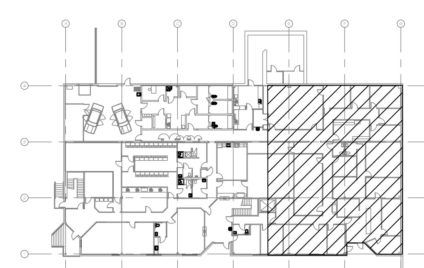
KEY PLAN 1 ST FLR
