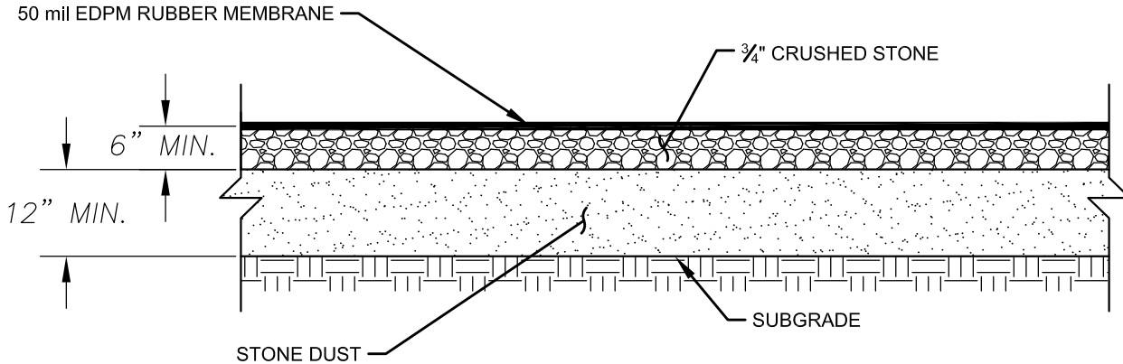
TRUCK WASHOUT PAD - SECTION VIEW NOT TO SCALE
