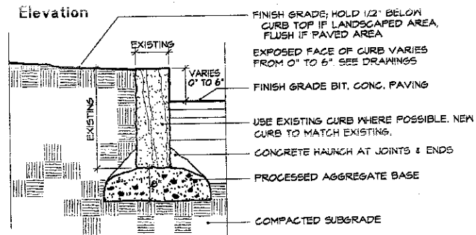
1 Granite Curb Not to Scale
