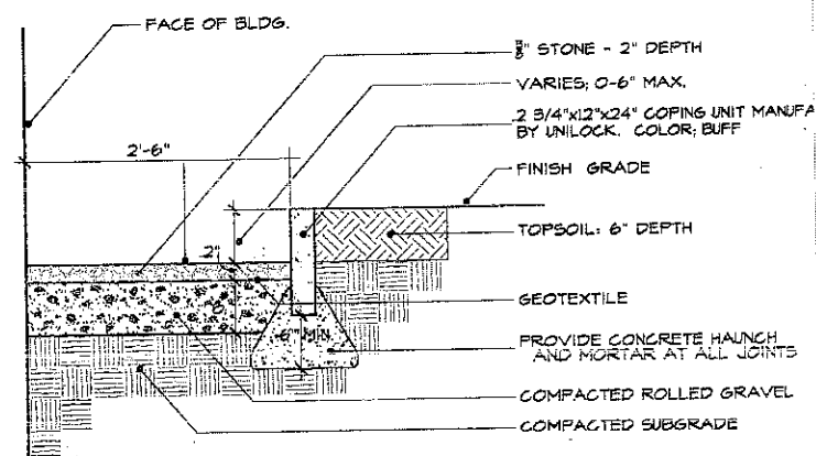
C Stone Drip Edge Not to Scale
