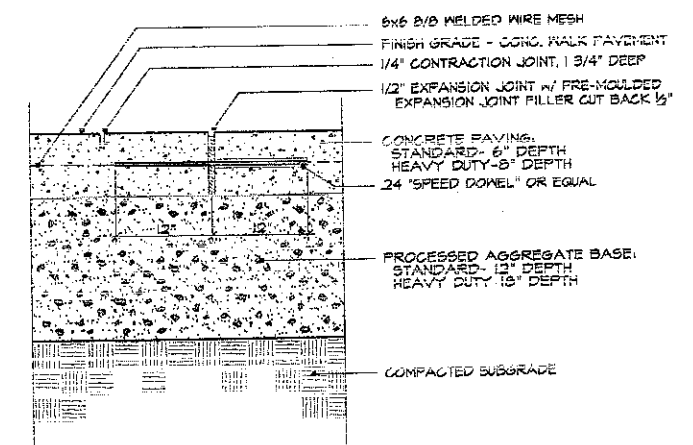
D1 D2 Concrete Paving-Standard(1)/Heavy Duty Not to Scale
