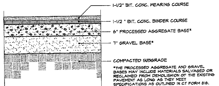
A Bituminous Concrete Paving-Standard Not to Scale
