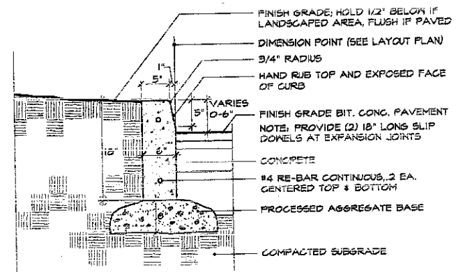
2 Cast Concrete Curb Not to Scale
