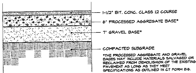
F Bituminous Concrete Walk Not to Scale
