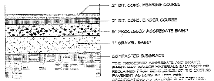
B Bituminous Concrete Paving-Heavy Duty Not to Scale
