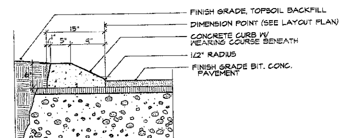
2 Cast Concrete Curb Not to Scale
