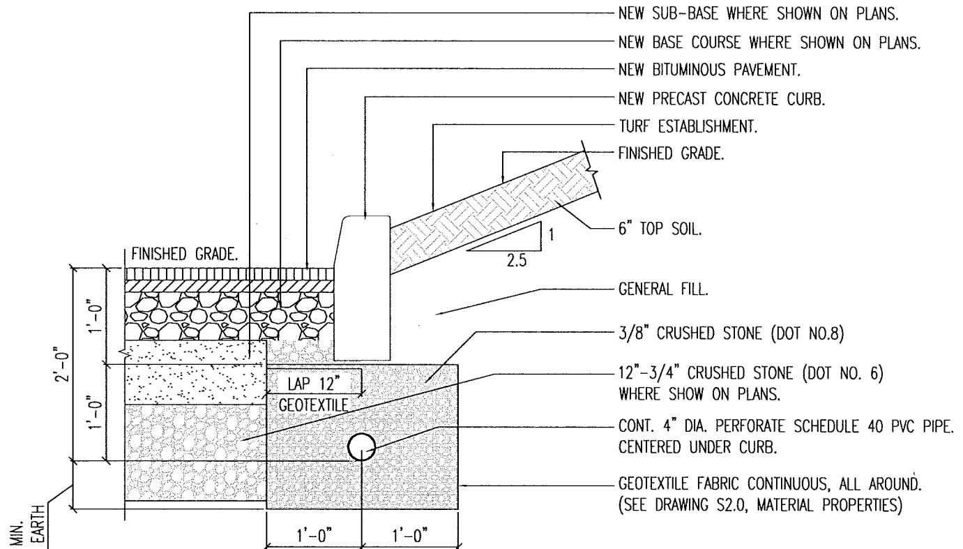
A TYPICAL EDGE OF PAVEMENT CONDITION
