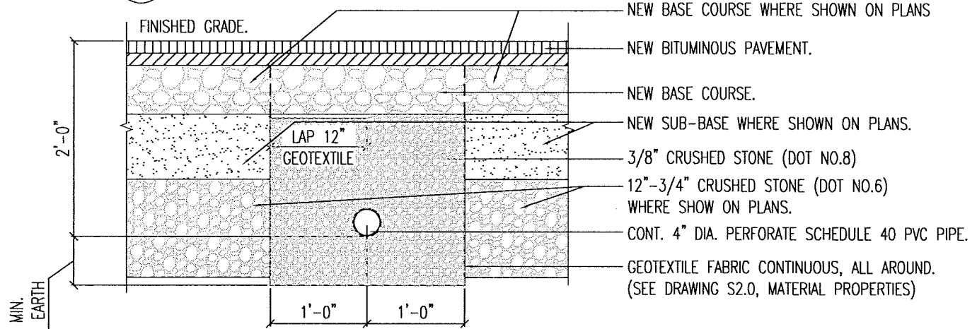
B TYPICAL INTERIOR PAVEMENT CONDITION
